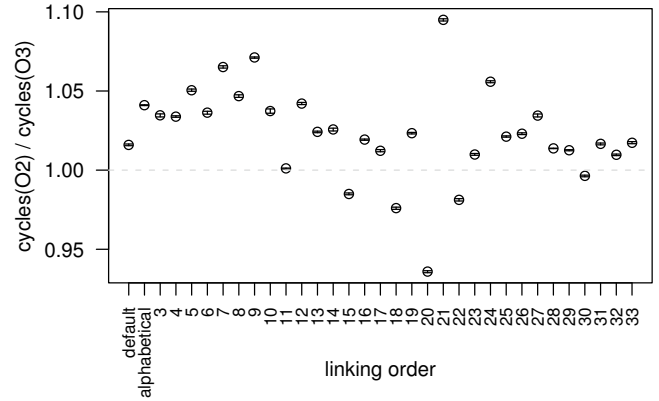
(a) Perlbench
