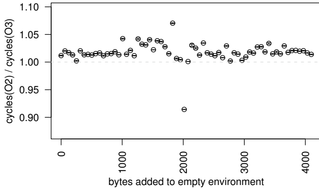
(a) Perlbench
